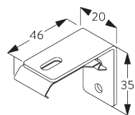
SG 2343 Support mural 46 mm
