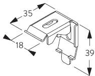
SG 2302 Support
