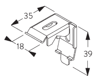
SG 2302 Support
