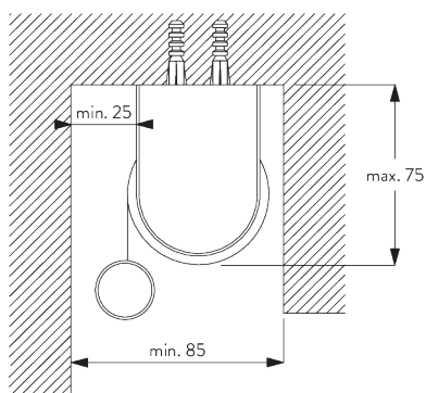
Supports SG 10873
