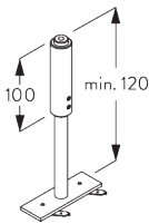
SG 6105 Suspension
